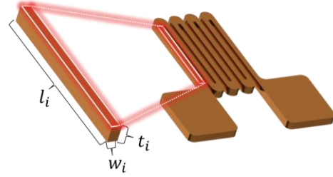
Figure 5. Schematic of discrete element in complicated gage pattern
