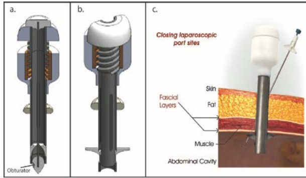
Figure 3: Cross-sectional view of trocar at a) Pre-insertion with wedges closed and obturator — a device used to penetrate the abdominal wall during the initial introduction of the trocar — in place, b) Surgery with inner tube down, wedges open, slits closed, and c) Closure with needle passing through opened slits.
