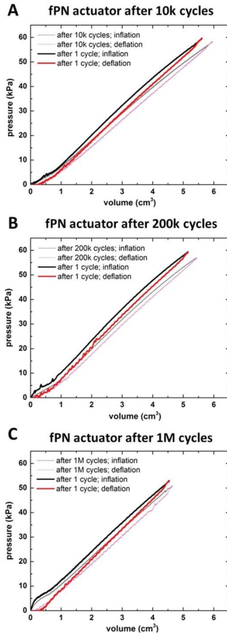
Figure 4. Fatigue test of fPN actuators. A–C) Pressure-volume hysteresis curves for fPN actuators before and after repeated pneumatic actuation. fPN actuators are made of Elastosil M4601 and paper and are hydraulically actuated to generate the PV curves.
