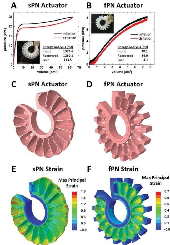
Figure 2. Comparison of fPN and sPN actuators. A,B) Pressure-volume hysteresis curves for actuators undergoing quasi-static hydraulic inflation/ deflation. The areas under the inflation and deflation curves signify the amount of energy added to and recovered from the actuator. Lost energy is the difference between the input and recovered energy. Inset images show actuators at the maximum inflation pressure. C–F) Simulated images, generated by a finite-element model, of the bending of the sPN (C,E) and fPN (D,F) actuators and the levels of the maximum principal strain (i.e., 1D dimensionless units) experienced by the actuator when fully pressurized.
