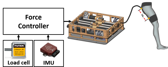
Fig. 2. Electromechanical sensing and control system. The timing of the motor force and position control profile is generated in real-time based on sensor input from thigh mounted IMU and load cell.
