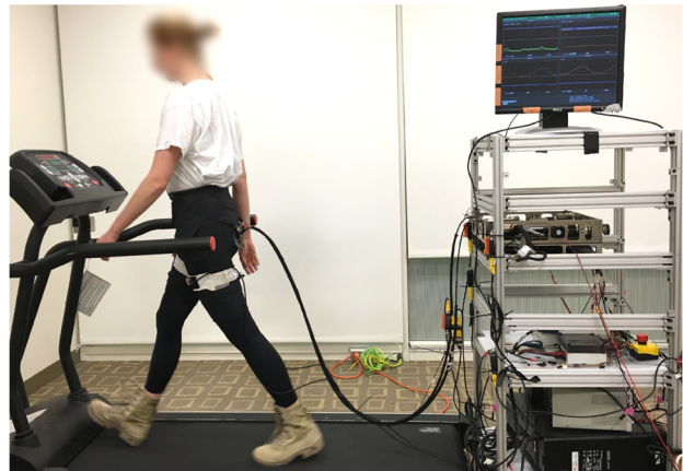
Fig. 1. Hip extension soft exosuit system. IMU measures thigh angles. Two sets of Bowden cables are connected between the multi-joint actuation platform and the exosuit to provide hip extension assistance during walking. The assistive force is transmitted from the multi-joint actuation platform to the wearer.
