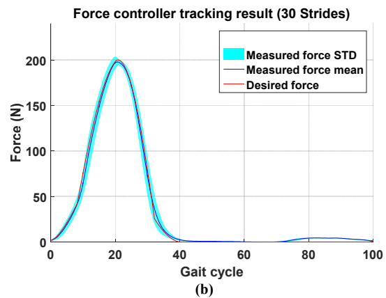
Fig. 2: Force tracking results using the position controller (a) and the force controller (b). The results were from a healthy participant at 1.35 m/s steady state walking for 30 strides.
