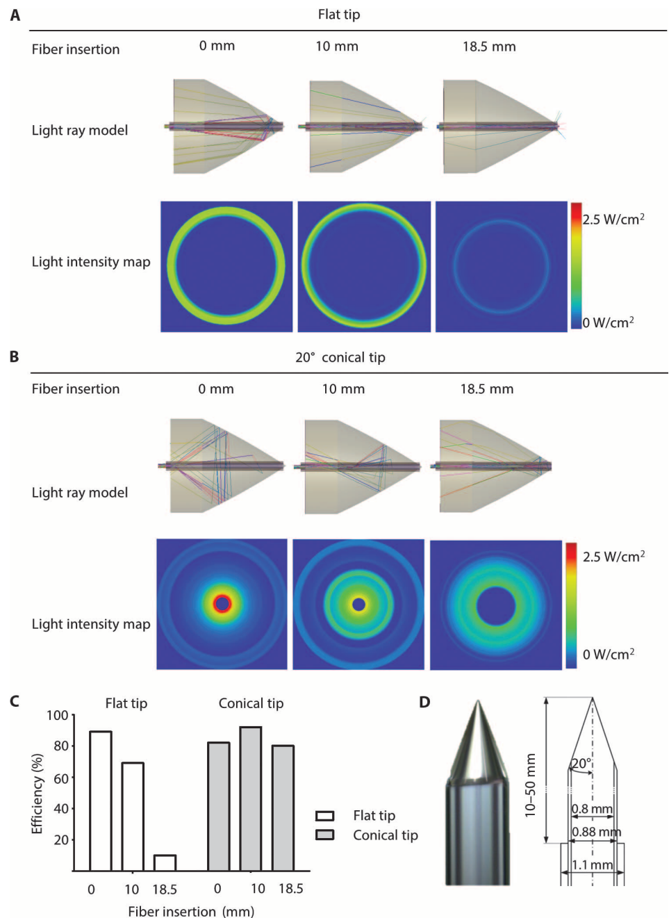
Fig. 3. Optimization of a low-profile fiber optic for light dispersion. (A and B) Light ray model and intensity map on the patch/septum for a flat-tip fiber (A) and a conical fiber (20° half-angle) (B) with an insertion distance into the balloon of 0, 10, and 18.5 mm. The images on the top of each panel trace a sample of random rays. The simulations in the bottom of each panel are based on 10^8 rays for a total launched power of 1 W. The efficiency calculations assumed that 100% of the light was available in the fiber before the light was launched into the catheter distances of 0, 10, and 18.5 mm. (C) Efficiency (total power at detector divided by input power) of flat and conical tips. Data are the results of the simulation ( n = 1 for each tip shape) at each catheter insertion distance. (D) Sculpted conical fiber optic tip and corresponding dimensions.
