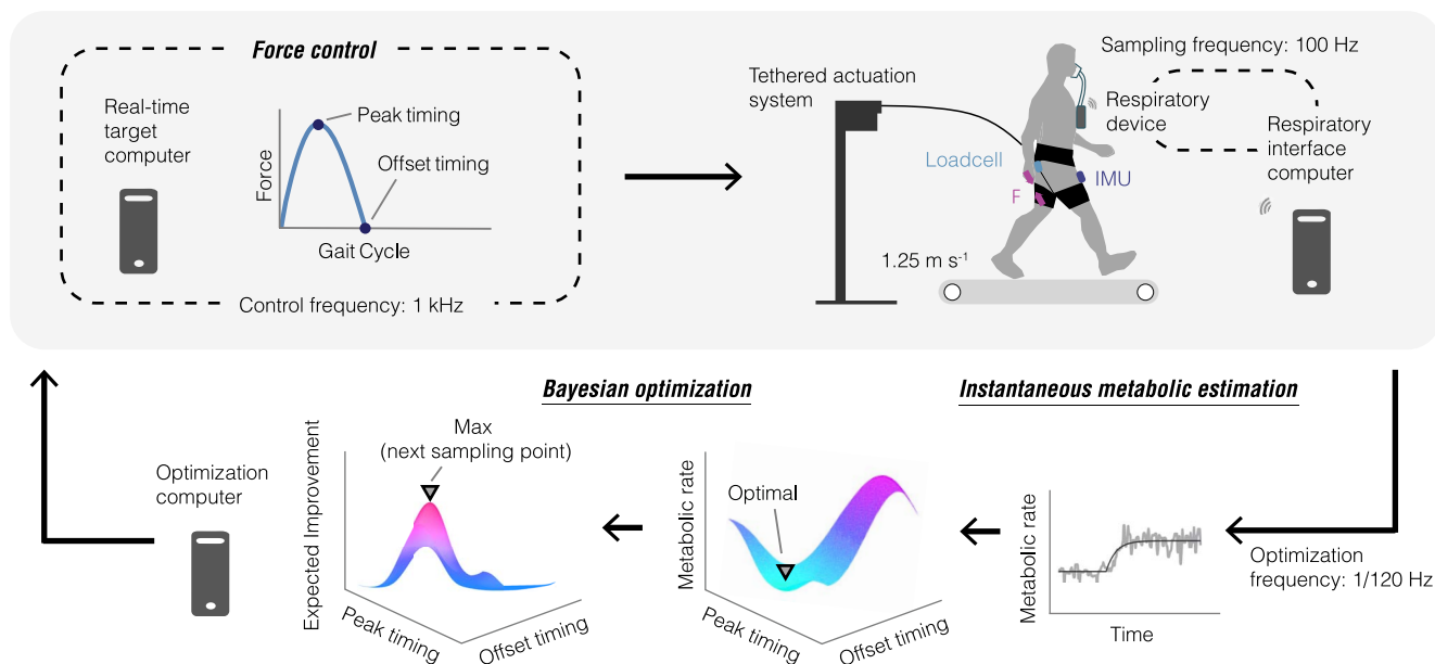
Fig. 1. Experimental setup for HIL Bayesian optimization. Bayesian optimization was used to adjust the control parameters of an assistive device to minimize the metabolic cost of walking. The metabolic rate was estimated from respiratory measurements and used to compute a posterior distribution of metabolic rate with respect to the free control parameters. The posterior was initially generated by evaluating six prefixed control parameters. Given the posterior at the current iteration, the control parameters with maximum EI were chosen and applied to the wearable device. This process was repeated until convergence. During this process, the configured force profiles were delivered through a soft hip exosuit with a tethered actuation system.
