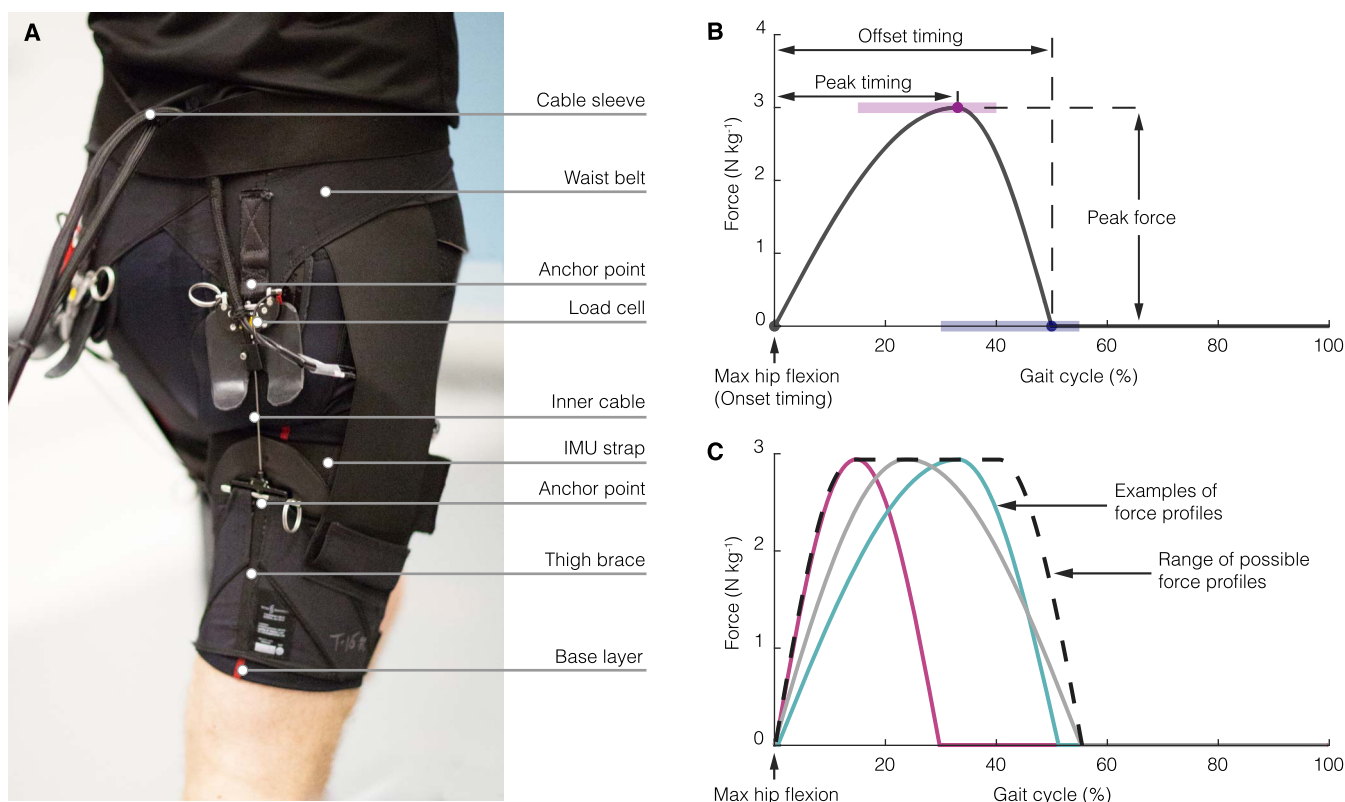
Fig. 2. Soft exosuit and assistive hip force profile. (A) The hip soft exosuit. A hip extension moment was generated by pulling the inner cable to create a tension between two anchor points. (B) Parameterization of hip force profile. The hip force profile was chosen to be a combination of two parameterized sinusoidal curves joined at the peak. Peak force was set to 30% of body weight, and onset timing was fixed to the time of maximum hip flexion. Peak and offset timing were actively adjusted by the optimization to determine the shape of the force profile as a function of gait percentage. Shaded purple and blue bars represent the range of peak and offset timing, respectively. (C) Examples of feasible hip force profiles.
