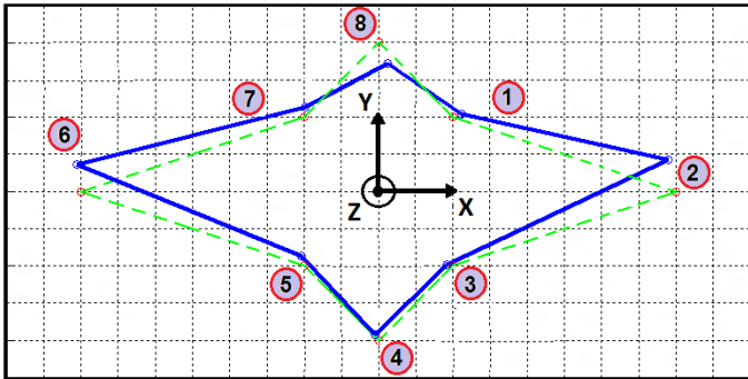
Figure 19. TARGETING RESULTS FROM EXPERIMENTS PERFORMED IN GELATIN (GRID SHOWN IN CM INTERVAL). THE PLANNED PATTERN IS SHOWN WITH DOTTED LINES, AND THE ACTUAL PATTERN IS SHOWN WITH SOLID LINES. ERROR VARIES FROM 0.9 MM TO 4.5MM FOR THE 8 TARGETS.
