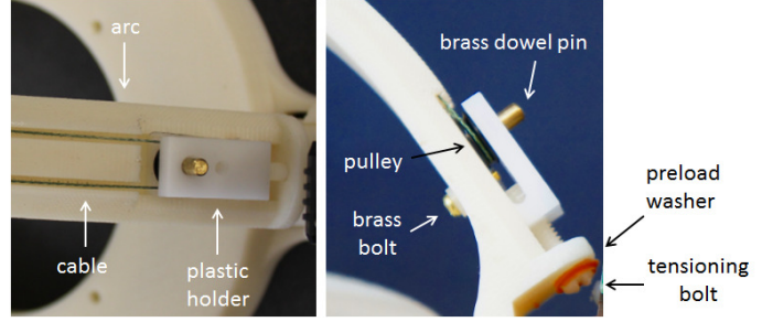
Figure 7. THE CABLE TENSIONING MECHANISM USES A BOLT TO FINE TUNE THE POSITION OF THE TENSIONING PULLEY AND ELIMINATE BACKLASH.
